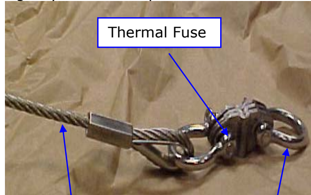
2' Cable from wheel supplied valve or kit
